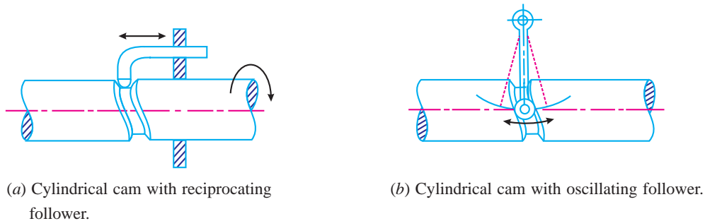
Fig. 20.2. Cylindrical cam.
