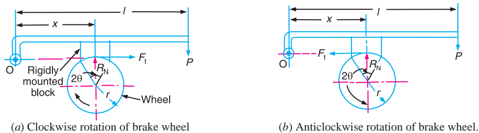
Fig. 19.1. Single block brake. Line of action of tangential force passes through the fulcrum of the lever.
