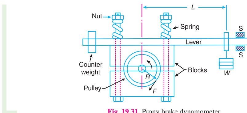
Fig. 19.31. Prony brake dynamometer.
