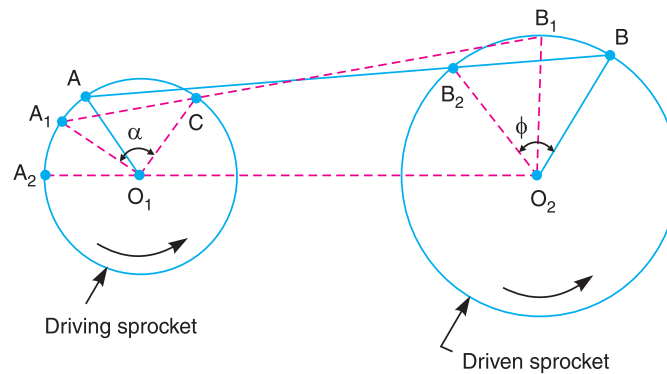
Fig. 11.27. Kinematic of chain drive.
