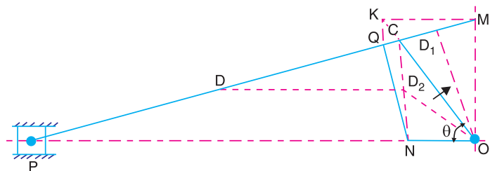
Fig. 15.3. Ritterhaus's construction.
