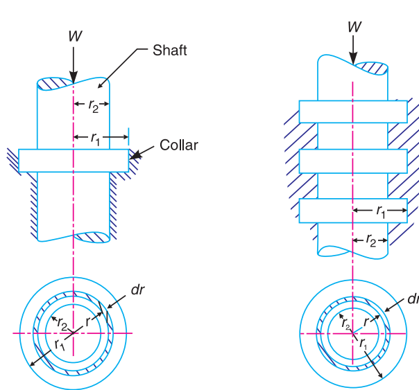
(a) Single collar bearing (b) Multiple collar bearing.
