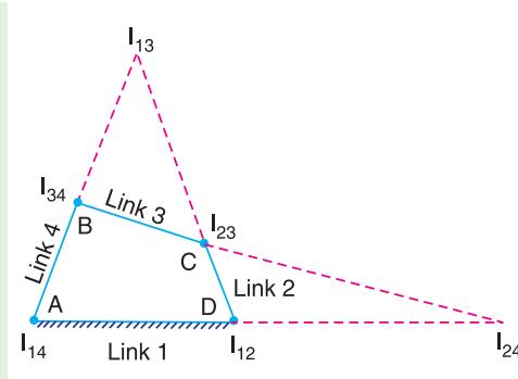
Fig. 6.5. Types of instantaneous centres.
