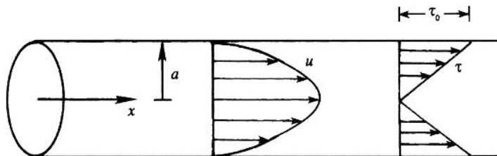
Figure 17.11 Poiseuille flow.
