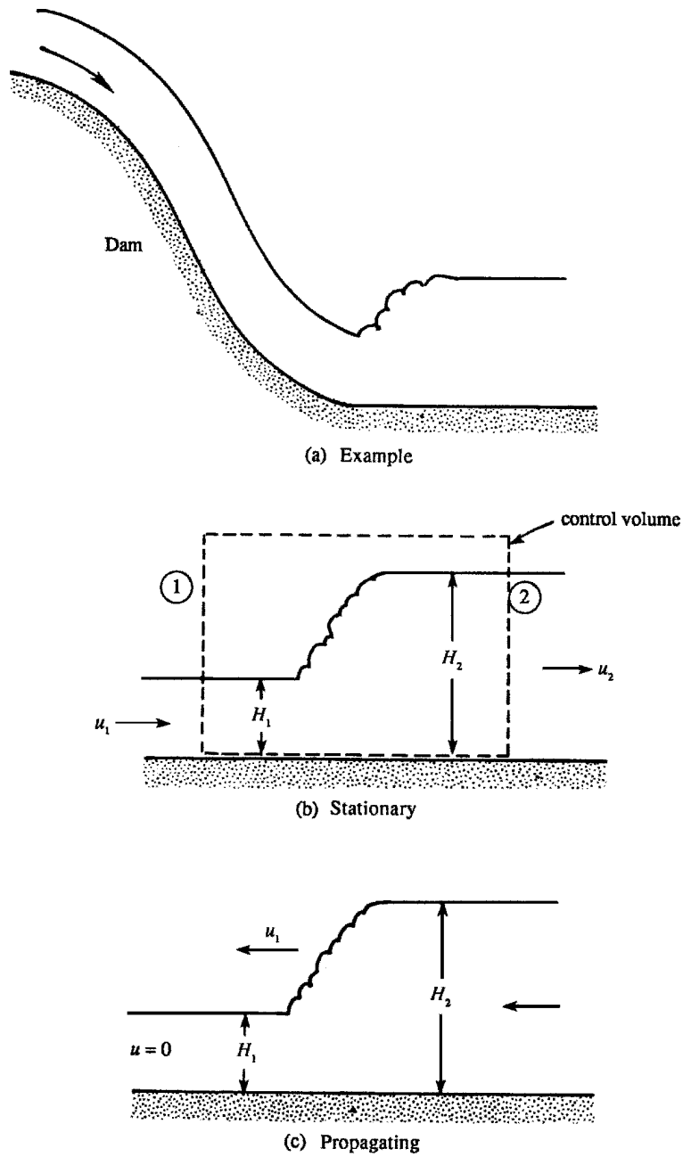
Figure 7.23 Hydraulic jump.
