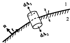
Figure 4.22 Interface between two media; evaluation of boundary conditions.
