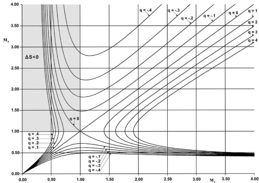
Figure 16.17 Flow in a constant-area duct with heating/cooling q as parameter; f = 0 . Upper left quadrant is inaccessible because \Delta S < 0 . \gamma = 1.4 .
