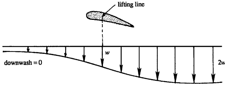
Figure 15.23 Variation of downwash ahead of and behind an airfoil.
