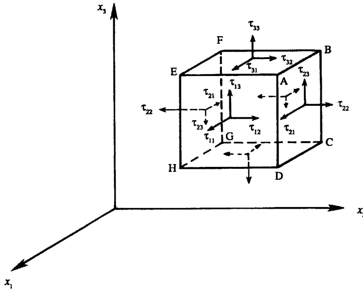
Figure 2.4 Stress field at a point. Positive normal and shear stresses are shown. For clarity, the stresses on faces FBCG and CDHG are not labeled.
