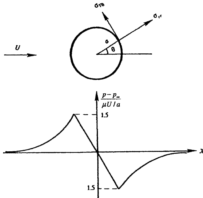
Figure 9.14 Creeping flow over a sphere. The upper panel shows the viscous stress components at the surface. The lower panel shows the pressure distribution in an axial ( \varphi = \text{const.} ) plane.
