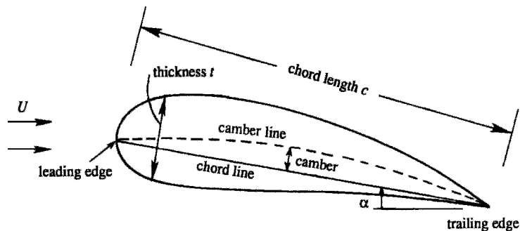
Figure 15.6 Airfoil geometry.
