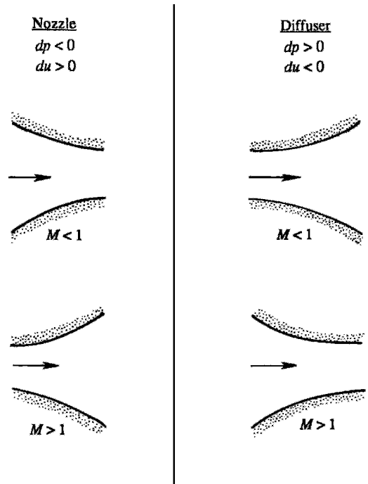
Figure 16.5 Shapes of nozzles and diffusers in subsonic and supersonic regimes. Nozzles are shown in the left column and diffusers are shown in the right column.
