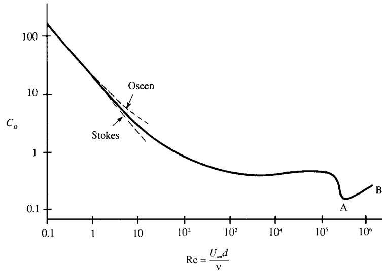
Figure 10.23 Measured drag coefficient of a smooth sphere. The Stokes solution is C_D = 24/Re , and the Oseen solution is C_D = (24/Re)(1 + 3Re/16) ; these two solutions are discussed in Chapter 9, Sections 12 and 13. The increase of drag coefficient in the range AB has relevance in explaining why the flight paths of sports balls bend in the air.
