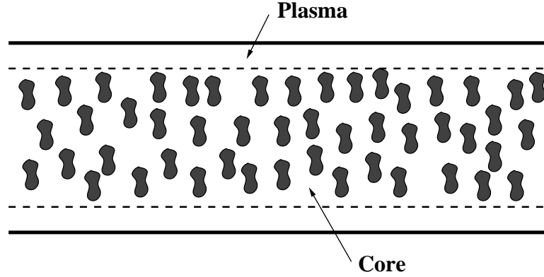
Figure 17.12 Fahraeus-Lindqvist effect.
