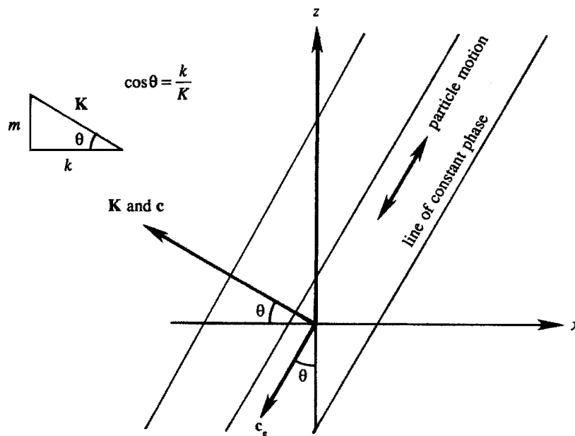
Figure 7.32 Basic parameters of internal waves. Note that \mathbf{c} and \mathbf{c}_g are at right angles and have opposite vertical components.
