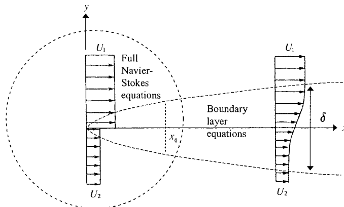
Figure 10.35 Decay of a laminar shear layer.
