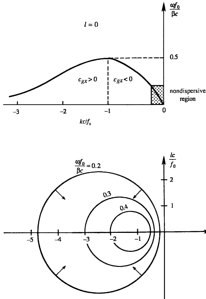
Figure 14.28 Dispersion relation \omega(k, l) for a Rossby wave. The upper panel shows \omega vs k for l = 0 . Regions of positive and negative group velocity c_{gx} are indicated. The lower panel shows a plan view of the surface \omega(k, l) , showing contours of constant \omega on a kl -plane. The values of \omega f_0 / \beta c for the three circles are 0.2, 0.3, and 0.4. Arrows perpendicular to \omega contours indicate directions of group velocity vector c_g . A. E. Gill, Atmosphere–Ocean Dynamics , 1982 and reprinted with the permission of Academic Press and Mrs. Helen Saunders-Gill.
