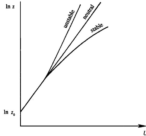
Figure 13.25 Effect of stability on velocity profiles in the surface layer.
