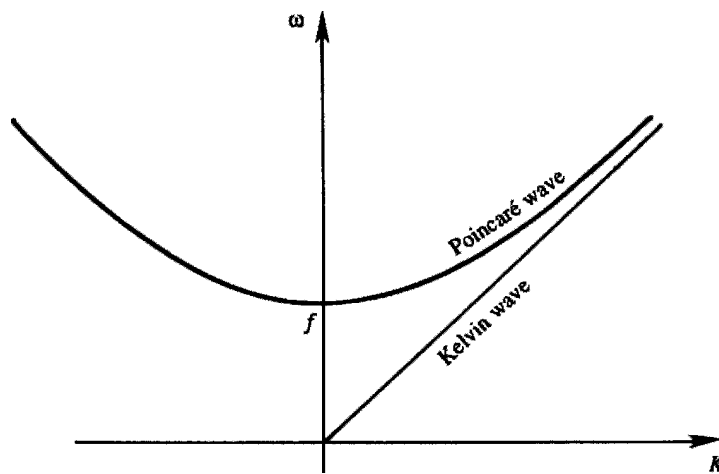
Figure 14.14 Dispersion relations for Poincaré and Kelvin waves.
