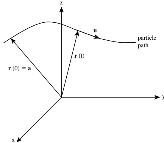
Figure 3.2 Particle—Lagrangian description. Independent variables: (\mathbf{a}, t) ; dependent variables: \mathbf{r}(\mathbf{a}, t) , \mathbf{u} = (\partial\mathbf{r}/\partial t)_{\mathbf{a}} , \rho = \rho(\mathbf{a}, t) , and so on.
