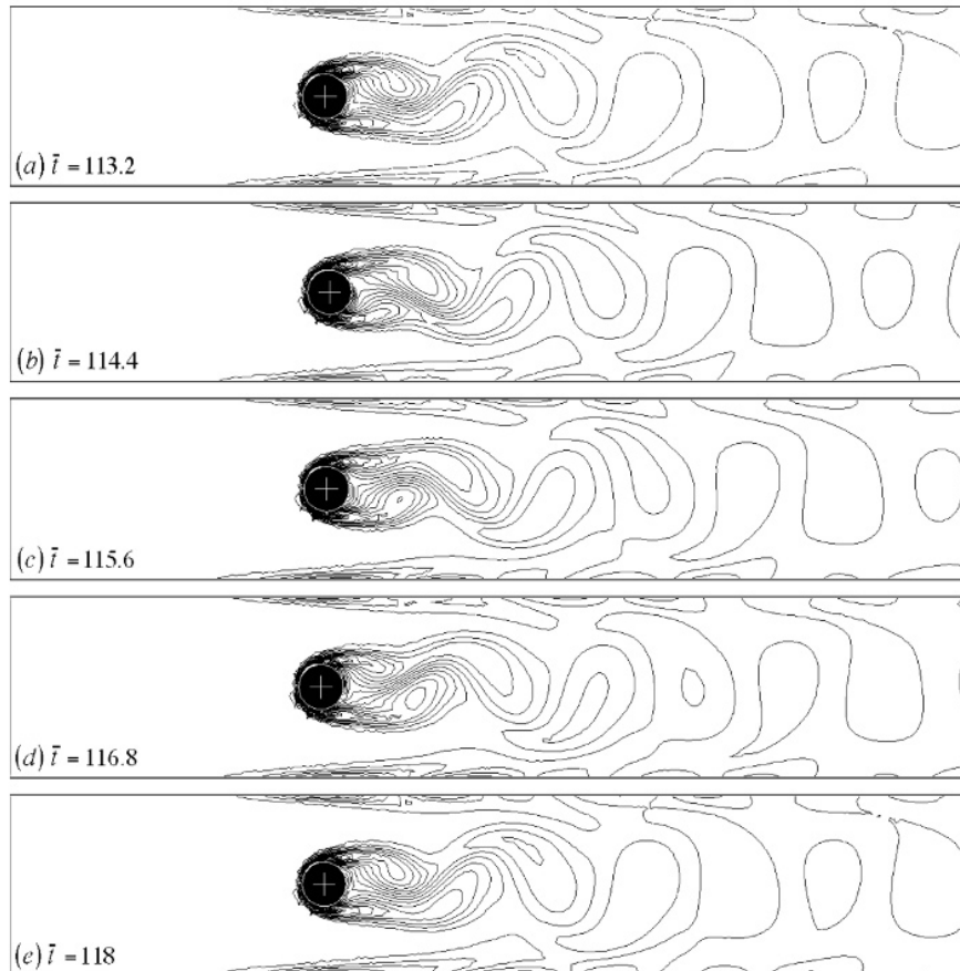
Figure 11.20 Vorticity lines for flow around a cylinder at Reynolds number Re = 100 . \tilde{t} = tU/d is the dimensionless time.
