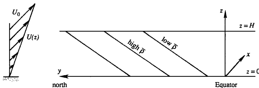
Figure 14.30 Lines of constant density in the northern hemispheric atmosphere. The lines are nearly horizontal and the slopes are greatly exaggerated in the figure. The velocity U(z) is into the plane of paper.
