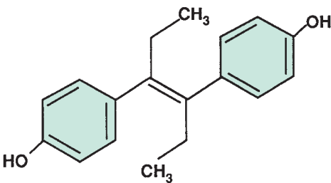
Diethylstilbestrol
