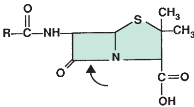
Penicillin nucleus
