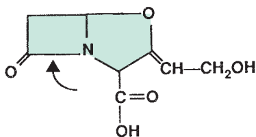
Clavulanic acid
