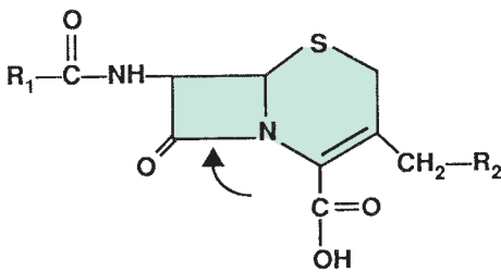
Cephalosporin nucleus
