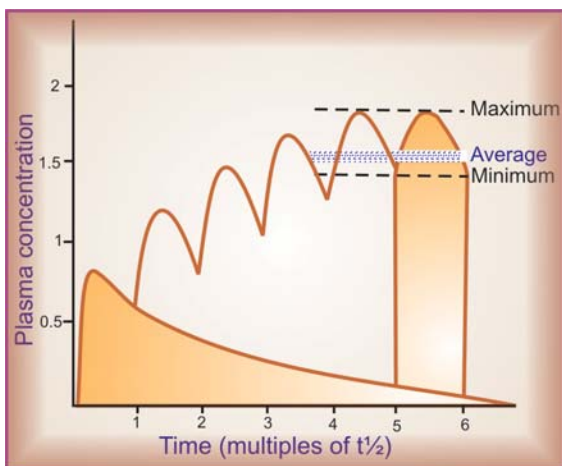
Fig. 3.6: Plateau principle of drug accumulation on repeated oral dosing.
