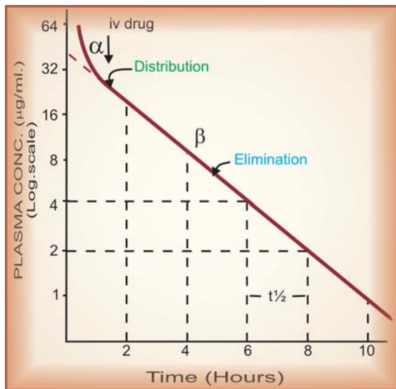
Fig. 3.4: Semilog plasma concentration-time plot of a drug eliminated by first order kinetics after intravenous injection
