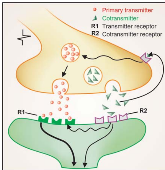
Fig. II.3: Cotransmission
